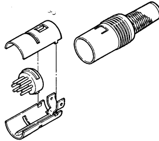
CONNECTOR ASSEMBLY
